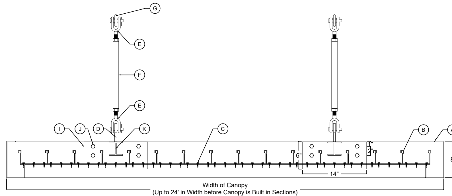
2 TRANSVERSE VIEW SCALE: 1" = 1'-0"
