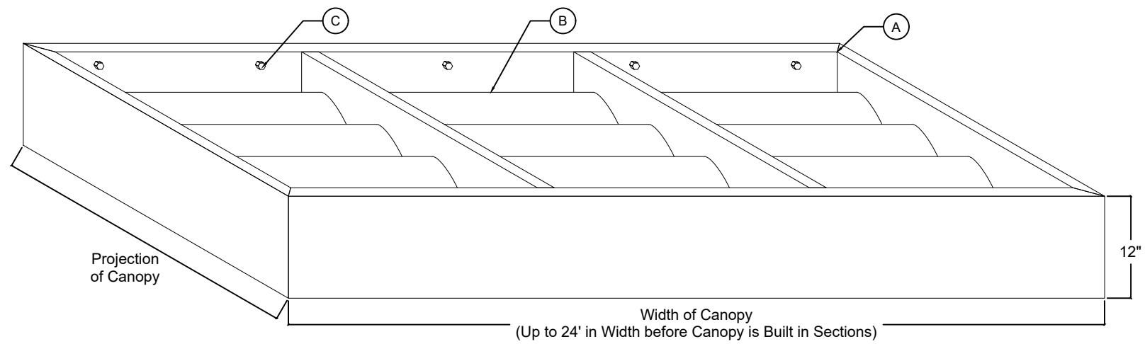
1 DIMENSIONAL VIEW SCALE: 3/4" = 1'-0"
