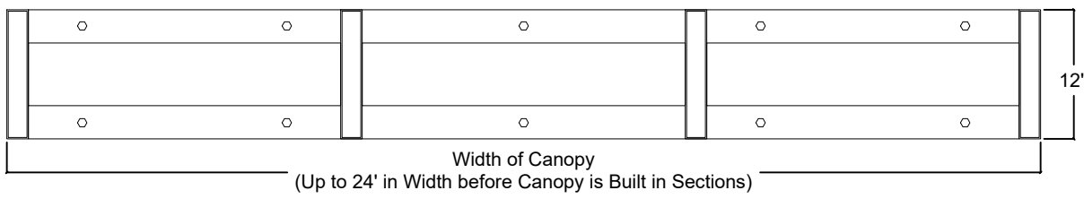
3 TRANSVERSE VIEW SCALE: 3/4" = 1'-0"
